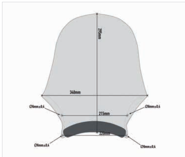
A200+ A4124A Kawasaki Z900RS (18 > 20) Universal screen, smoked 29,5 x 34 cm
